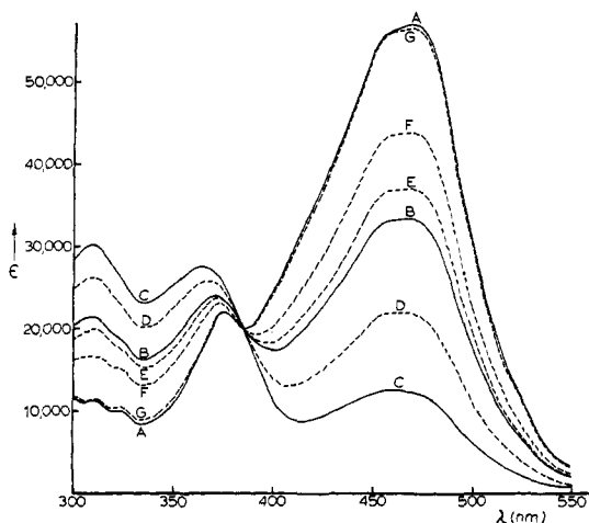
Figure 4. Spectral changes during irradiation (—) ( \lambda > 500 nm) and after irradiation (---) of a degassed solution of thione in \text{CH}_2\text{Cl}_2 at 0.4^\circ . Irradiation time (sec): A, 0; B, 5; C, 525. Time after irradiation (nm): D, 10; E, 30; F, 50; G, 200.
